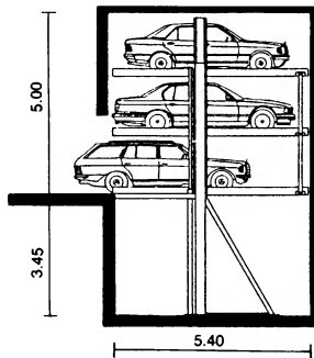
④ Private parking, 2 cars stacked vertically
